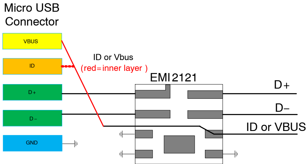
Figure 15. EMI2121 Micro - USB Connector Application Diagram
